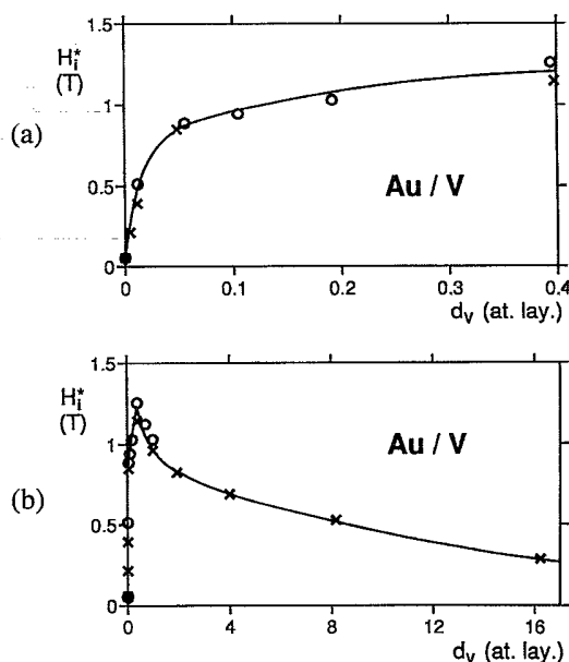
FIG. 2. The dephasing field (which is proportional to 1/\tau_i + 2/\tau_s ) as a function of the V thickness: (a) for small V thickness, (b) for the whole thickness range.
