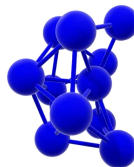
Fig. 1 Optimized icosahedral pocket structure using DFT (PBE0/ecp-10-mdf (Ni))
