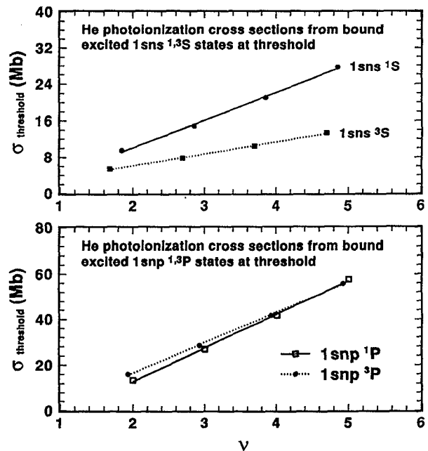
FIG. 3. Total \sigma_{\text{threshold}} from bound excited 1sns 1,3S and 1snp 1,3P states as a function of the effective principal quantum numbers \nu .
