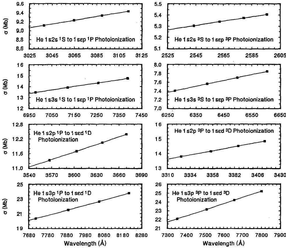
FIG. 2. Absolute cross sections for a few selected 1,3S \rightarrow 1,3P and 1,3P \rightarrow 1,3D photoionizations. The solid lines are fitted to the calculated values labeled by the solid squares.
